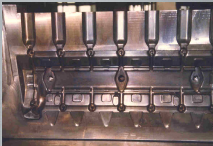
Coquilla grande estructural carter motor MWM.
